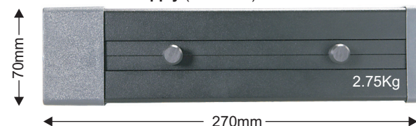
2022 Power Supply (side view)
